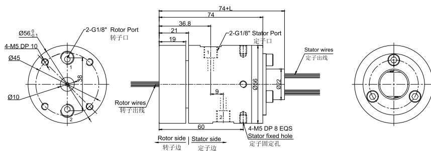
MKD21S-S06(S12,S18,S24,S36)尺寸图, 2进2出G1/8"牙+06~36路信号(2A)
